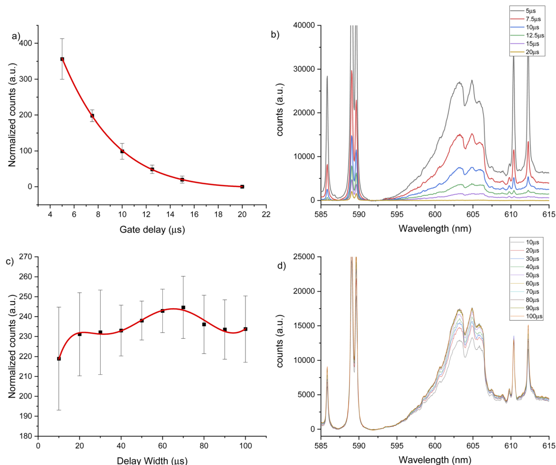
Fig. 5 LIBS signal optimization under helium flow of 1 L min -1 for 600 nm window using a 2500 μg g -1 hydroxyapatite standard. (a) Gate delay optimization maintaining constant gate width at 50 μs, (b) LIBS spectrum for each gate delay change, (c) gate width optimization maintaining constant gate delay at 10 μs, (d) LIBS spectrum for each gate width change.
