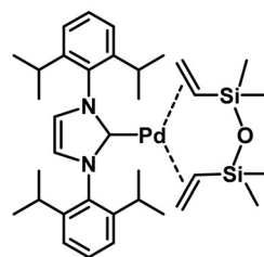
Fig. 4 Other ligand development for the palladium-catalyzed telomerization of 1,3-butadiene with methanol.
