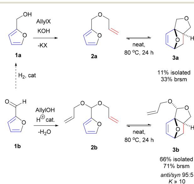
Scheme 1 Intramolecular DA cycloadditions with furfural allyl ether 2a /furfural diallyl acetal 2b ; brsm = based on recovered starting material.
