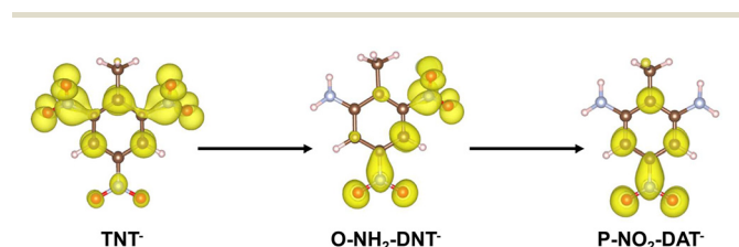
Fig. 3 Isodensity surface for electron in the highest occupied molecular orbital (HOMO) for TNT − , O-NH 2 -DNT − , and P-NO 2 -DAT − anion species. Atom colors are presented as brown: C, white: H, blue: N, and red: O. A consistent isosurface level value (approximately 0.003) was used to construct the isodensity surfaces.
