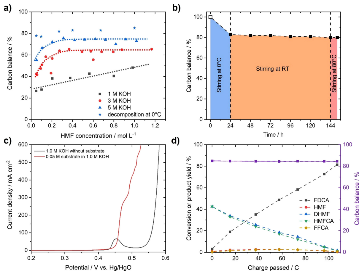
Fig. 2 HMF decomposition at different concentrations of HMF and KOH, and temperatures. Results are measured after 20 h. The determined carbon balance is based on the sum of HMF, DHMF and HMFCa present in the solution. Dashed lines are used as a guide to the eyes. (b) Stability measurement of a 1 M HMF solution in 5 M KOH. Decomposition of HMF to the Cannizzaro products, DHMF and HMFCa, was performed at 0 °C during the first 24 h. After 120 h of stirring at RT, temperature stability was evaluated by stirring the solution for 8 h at 80 °C. Quantification was performed using qNMR with DMSO as an internal standard. 100% is based on the initial mass of HMF and assumed to be the starting point at t = 0 h. (c) LSV curves measured with and without 0.05 M of the resulting Cannizzaro products in 1 M KOH after decomposition (scan rate: 5 mV s -1 ). Potentials are corrected for the uncompensated solution resistance. (d) Reaction intermediates monitored for the oxidation of a 0.05 M solution of the Cannizzaro products (based on initial HMF input) in 1 M KOH during constant potential electrolysis (0.50 V vs. Hg/HgO) for 15 min.
