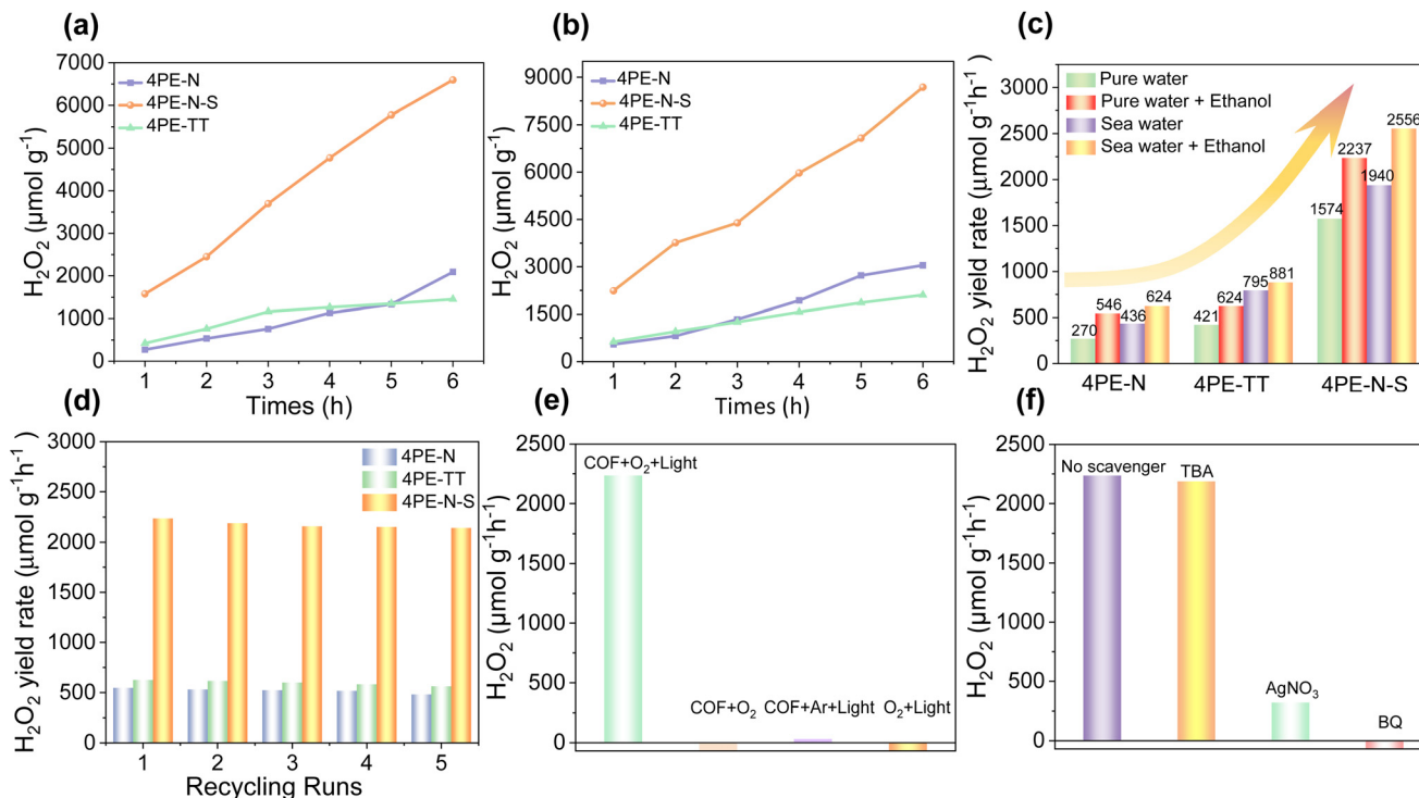
Fig. 4 Photocatalytic production of \text{H}_2\text{O}_2 for 4PE-N, 4PE-N-S, and 4PE-TT COFs under the illumination of a 300 W Xe lamp: (a) pure water, (b) water : ethanol (9 : 1) system, (c) comparison of \text{H}_2\text{O}_2 production among the photocatalysts with pure water and real seawater with and without ethanol. The photocatalytic performance of three COFs with one-hour of irradiation, (d) \text{H}_2\text{O}_2 production for five consecutive cycles using three COFs, (e) under different reaction conditions, (f) effects of scavengers ( 2 \text{ mmol L}^{-1} , 5 mg of photocatalyst, water : ethanol (9 : 1).
