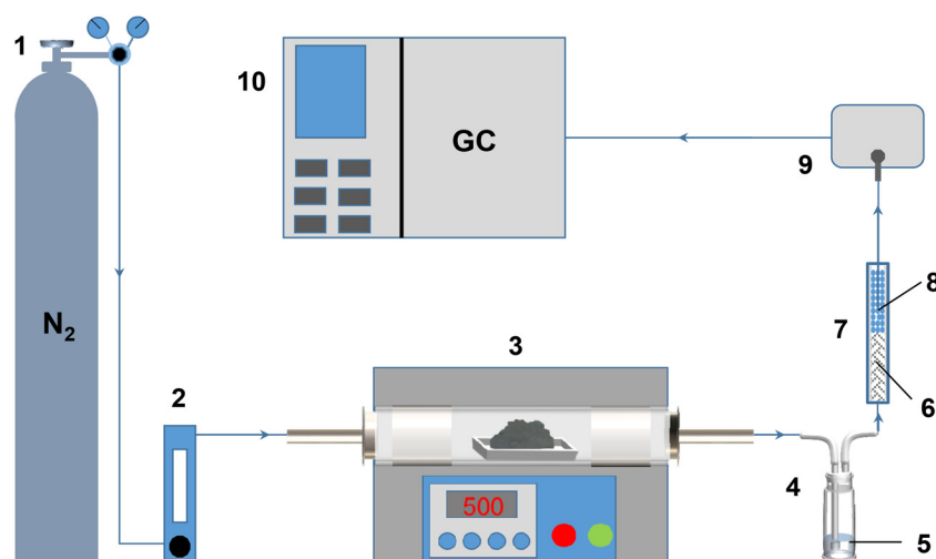
Fig. 1 The self-designed equipment for the thermochemical experiment (1. Nitrogen cylinder, 2. Gas flowmeter, 3. Glass tube furnace, 4. Gas-washing system, 5. Saturated sodium bicarbonate, 6. Skimmecotton, 7. Drying tube, 8. Discolored silica gel, 9. Gas sample collection bag, 10. Gas chromatograph instrument).
