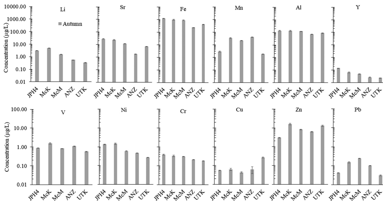
Fig. 7 Concentrations of selected TEs (ng L -1 ) in the porewaters of peat bogs, collected in autumn.
