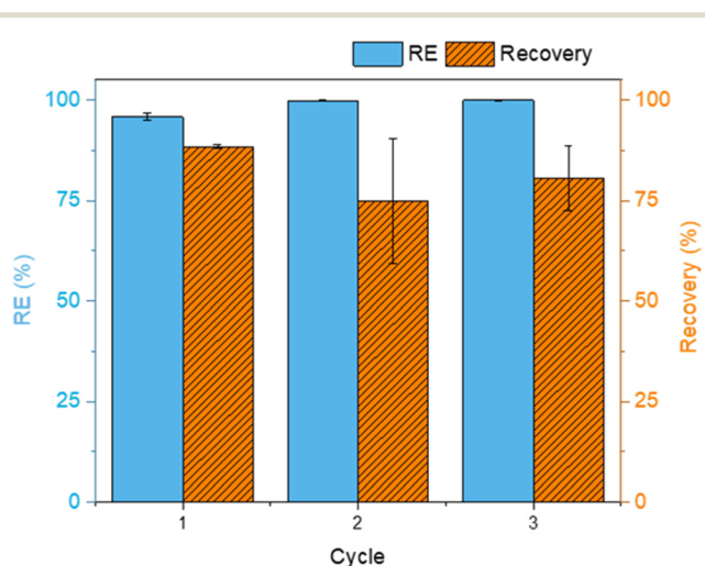
Fig. 8 Adsorption removal efficiency (blue) and desorption recovery (orange) for three cycles of regeneration of FLG@TA@RSN adsorbent. For adsorption, a BaP aqueous solution of 10 \mu\text{g L}^{-1} was prepared with 1% ethanol. An adsorption experiment was performed using 5 mg L -1 CN adsorbent for 15 min. For desorption, 2 mL of acetonitrile was used and desorption was performed for 10 min in an ultrasound bath. The vertical error bars correspond to the standard deviation determined from the two replicates. The removal efficiencies of the adsorption experiments were corrected for glassware adsorption based on blank experiments performed (see Fig. S7†).
