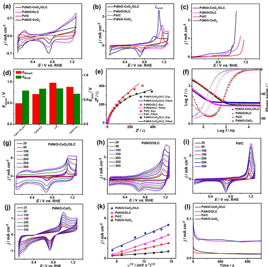
Fig. 3 CV profiles at 50 mV s -1 in (a) N 2 -saturated HClO 4 (0.1 M) and (b) CO-saturated HClO 4 (0.1 M). (c) LSV at 50 mV s -1 . (d) E_{Onset} and E_{Oxid} . (e) Nyquist plots. (f) Bode plots. (g–j) Scan rate studies. (k) Randles-Sevcik plots ( j_{Anode} vs. v^{1/2} ). (l) CA of PdNiO-CeO 2 /OLC, PdNiO/OLC, PdNiO-CeO 2 , and Pd/C in CO-saturated HClO 4 (0.1 M).
