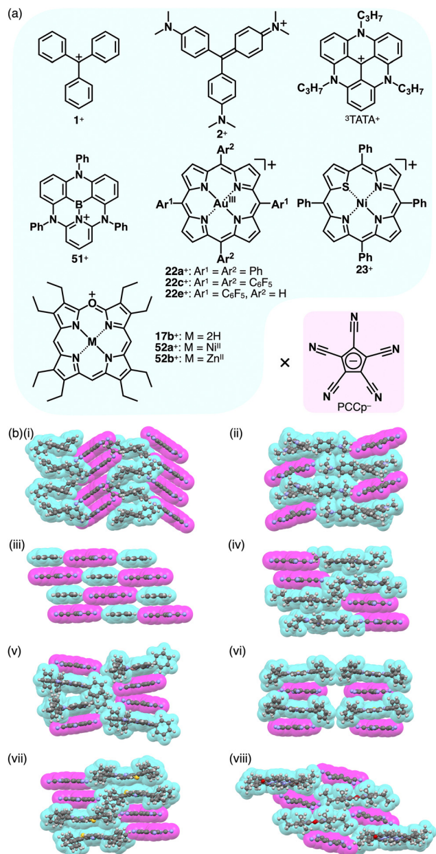
Fig. 34 (a) Combinations of \pi -electronic ion pairs: \text{PCCp}^{-} with 1^{+} , 2^{+} , ^3\text{TATA}^{+} , BN-TATA 51^{+} , 22a,c,e^{+} , 23^{+} , 17b^{+} and 52a,b^{+} and (b) single-crystal X-ray structures of (i) 1^{+}\cdot \text{PCCp}^{-} , (ii) 2^{+}\cdot \text{PCCp}^{-} , (iii) \text{Tr}^{+}\cdot \text{PCCp}^{-} , (iv) ^3\text{TATA}^{+}\cdot \text{PCCp}^{-} , (v) 51^{+}\cdot \text{PCCp}^{-} , (vi) 22a^{+}\cdot \text{PCCp}^{-} , (vii) 23^{+}\cdot \text{PCCp}^{-} and (viii) 52b^{+}\cdot \text{PCCp}^{-} (redrawn from cif files: 227124, 1431734, 1431733, 1431735, 2063989, 1877990, 2167304 and 2144318). Atom colour code in (viii): violet in the ball-and-stick models refers to zinc.
