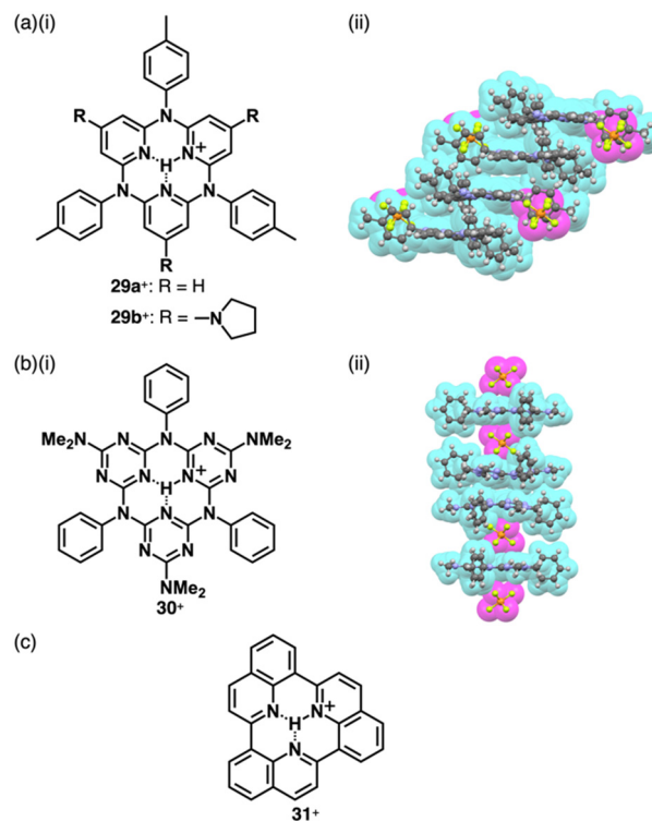
Fig. 19 (a) (i) Protonated azacalix[3](2,6)pyridine 29\text{a,b}^+ and (ii) single-crystal X-ray structure of 29\text{a}^+ -PF _6^- (redrawn from a cif file: 298963), (b) (i) protonated azacalix[3]triazine 30^+ and (ii) single-crystal X-ray structure of 30^+ -PF _6^- (redrawn from a cif file: 2072959) and (c) protonated triquinoline 31^+ .
