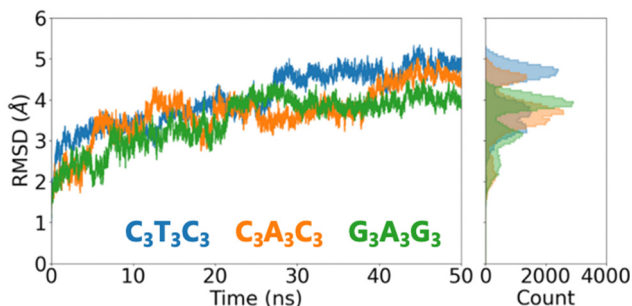
Fig. 2 RMSD change within 50 ns of MD simulation together with the RMSD histogram which shows RMSD mean and variation for each sequence.
