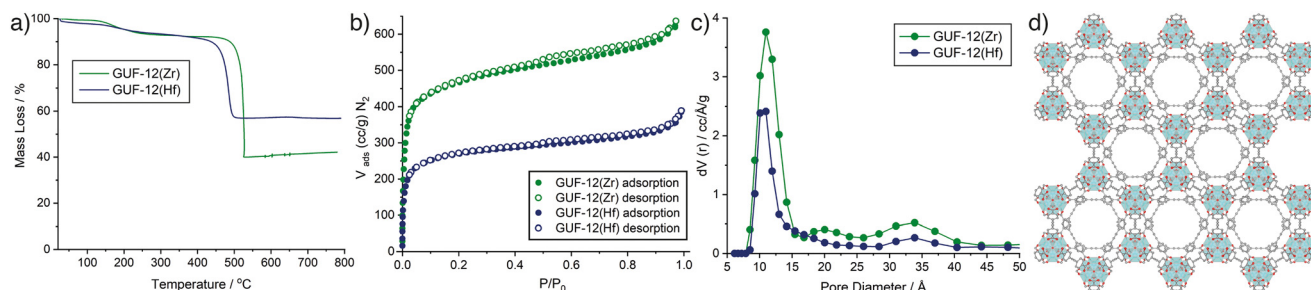
Fig. 4 a) Thermogravimetric analyses of GUF-12(Zr) and GUF-12(Hf) in air. b) N 2 adsorption-desorption isotherms (77 K) of GUF-12(Zr) and GUF-12(Hf) with c) pore-size distributions (N 2 at 77 K on carbon, slit pore, QSDFT, equilibrium model) calculated from the isotherms. d) Portion of the DFT model structure of GUF-12(Zr) viewed down the crystallographic c axis to visualise the hexagonal channel 11 Å in diameter.
