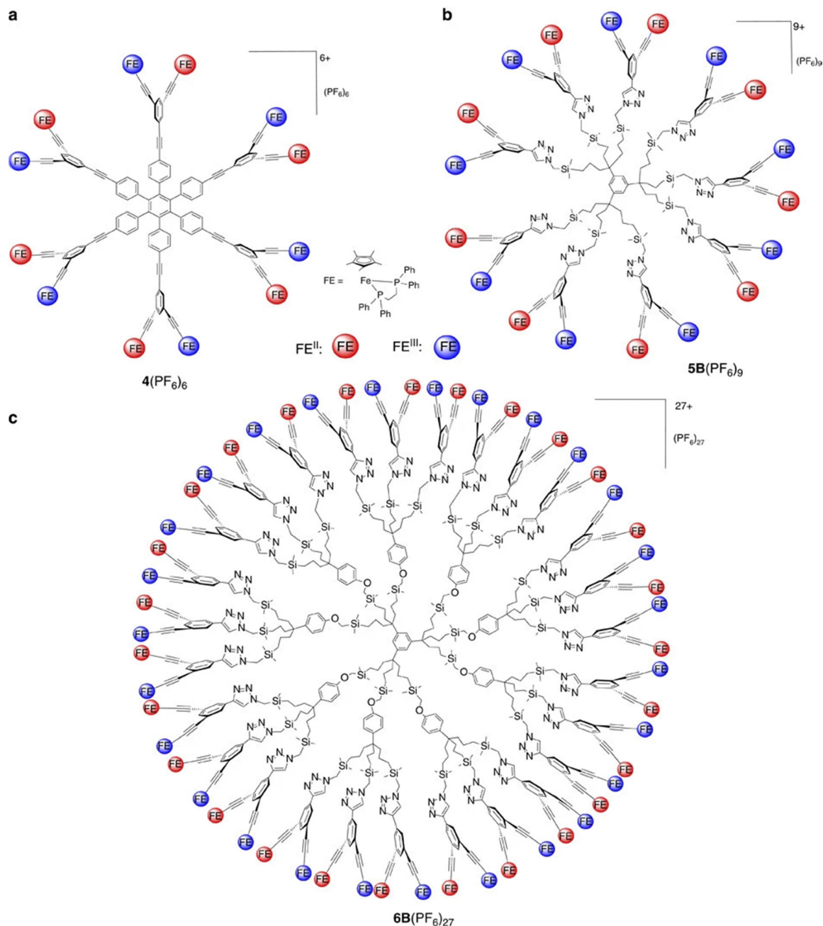
Fig. 6 Dendritic class-II mixed valence complexes synthesized by selective oxidation with ferricinium or comproportionation as shown in Scheme 9. Reproduced with permission from ref. 76 Copyright 2016 Springer Nature.
