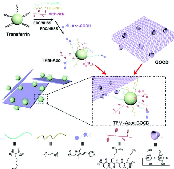
Fig. 20 Synthesis of the TPM-Azo guest, the GOCD host, and the TPM-Azo ⊂ GOCD host-guest supramolecular nanoassemblies. Reproduced with permission from ref. 114. Copyright 2019 The Royal Society of Chemistry.
