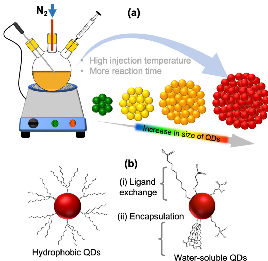
Fig. 3 (a) A typical setup for the synthesis of colloidal QDs, and (b) the schematic illustration of the procedure of surface modification of QDs showing: (i) ligand exchange of the hydrophobic ligands with water-soluble ones and (ii) encapsulation of hydrophobic QDs with hydrophilic polymers and silica coatings.
