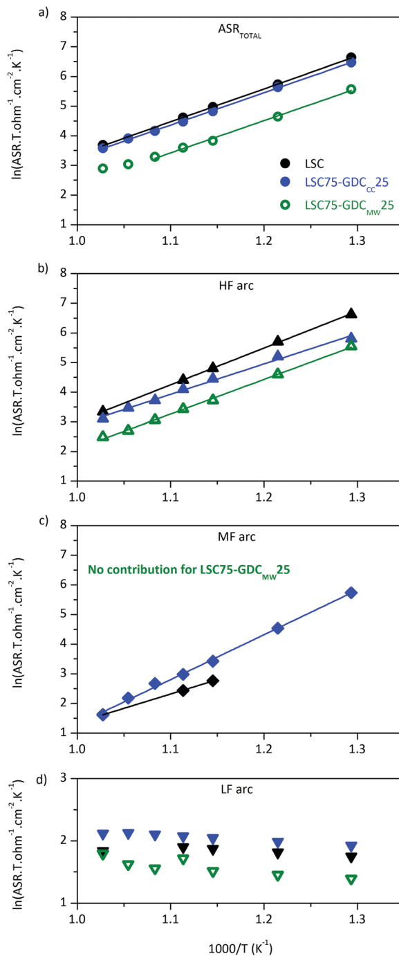
Fig. 6 Comparison of the electrochemical performance of LSC, LSC75-GDC CC25 and LSC75-GD MW25 cathodes between 500 and 700 °C. Arrhenius plots for (a) ASR_{TOTAL} ; (b) ASR_{HF} ; (c) ASR_{MF} and (d) ASR_{LF} . The colours correspondence to each sample is inserted in panel (a). Straight lines are the linear regression for the experimental data. Dashed line in panel (a) represents the extrapolation of the linear regression and spots the departure of the experimental data from the straight line at T > 650 °C.
