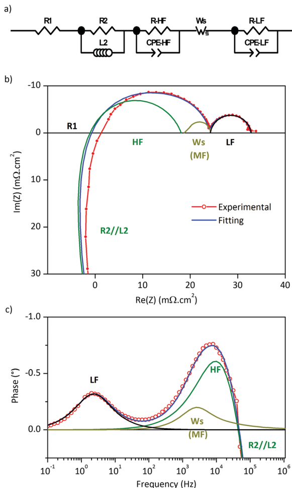
Fig. 5 Equivalent circuit analysis of EIS spectrum of LSC75-GDC CC25 cathode at 700 °C under synthetic air flow. (a) Scheme of the equivalent circuit used to fit the spectrum. (b) Normalized Nyquist plot and (c) bode phase diagrams of the experimental data along with the fitting function. In (b) and (c) it is also included the contribution of each circuit element to the fitting curve. In (b) the contribution of R_1 element was subtracted from the experimental data and fitting function.
