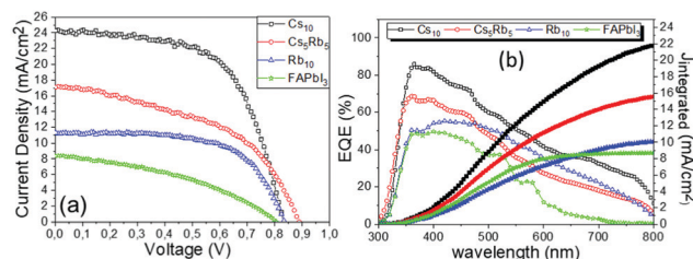
Fig. 3 (a) Current density–voltage curves of the champion C-PSCs, incorporating the MA-free perovskites under study, the under illumination of 100\text{ mW cm}^{-2} simulated sun irradiation (1.5 AM) and (b) EQE of the corresponding solar cells.
