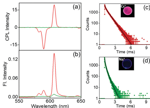
Fig. 4 (a) CPL and (b) fluorescence spectra of Cs^+[Eu((+)-tfac)_4]^- (red traces) and Na^+[Eu((+)-tfac)_4]^- (green traces) embedded in the PMMA films. (c and d) Luminescence lifetime plots of the hybrid PPMA films composed of (c) Cs^+[Eu((+)-tfac)_4]^- and (d) Na^+[Eu((+)-tfac)_4]^- ( \lambda_{ex} = 352 nm). The inset shows the photographs of the corresponding films collected upon excitation using a 365 nm UV lamp.
