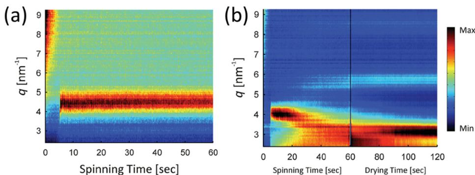
Fig. 20 Evolution of GIWAXS signal during film formation of (a) p -DTS(FBTT) 2 :PC 71 BM without DIO, which showed a rapid film formation, and (b) with 0.4 v% DIO, where a metastable polymorph was initially formed and gradually transformed to a different structure. Adapted with permission. 29 Copyright 2013, Wiley-VCH Verlag GmbH & Co. KGaA, Weinheim.
