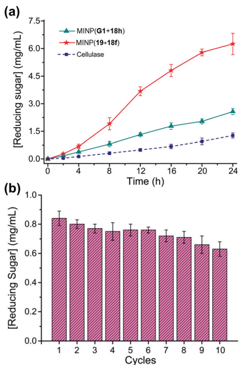
Fig. 10 (a) Comparison of reducing sugar formed during hydrolysis of cellulose by the synthetic MINP catalysts in 2 : 8 [C 2 mim]OAc/DMSO with 5% H 2 O at 90 °C and natural cellulase in NaOAc buffer pH 5.0 at 37 °C. [Cellulose] = 8 mg mL -1 . [Catalyst] = 2 mg mL -1 . (b) Recyclability of MINP( 19 + 18f ) on magnetic nanoparticles for cellulose hydrolysis. (Adapted with permission from ref. 79. Copyright 2021, the American Chemical Society.)
