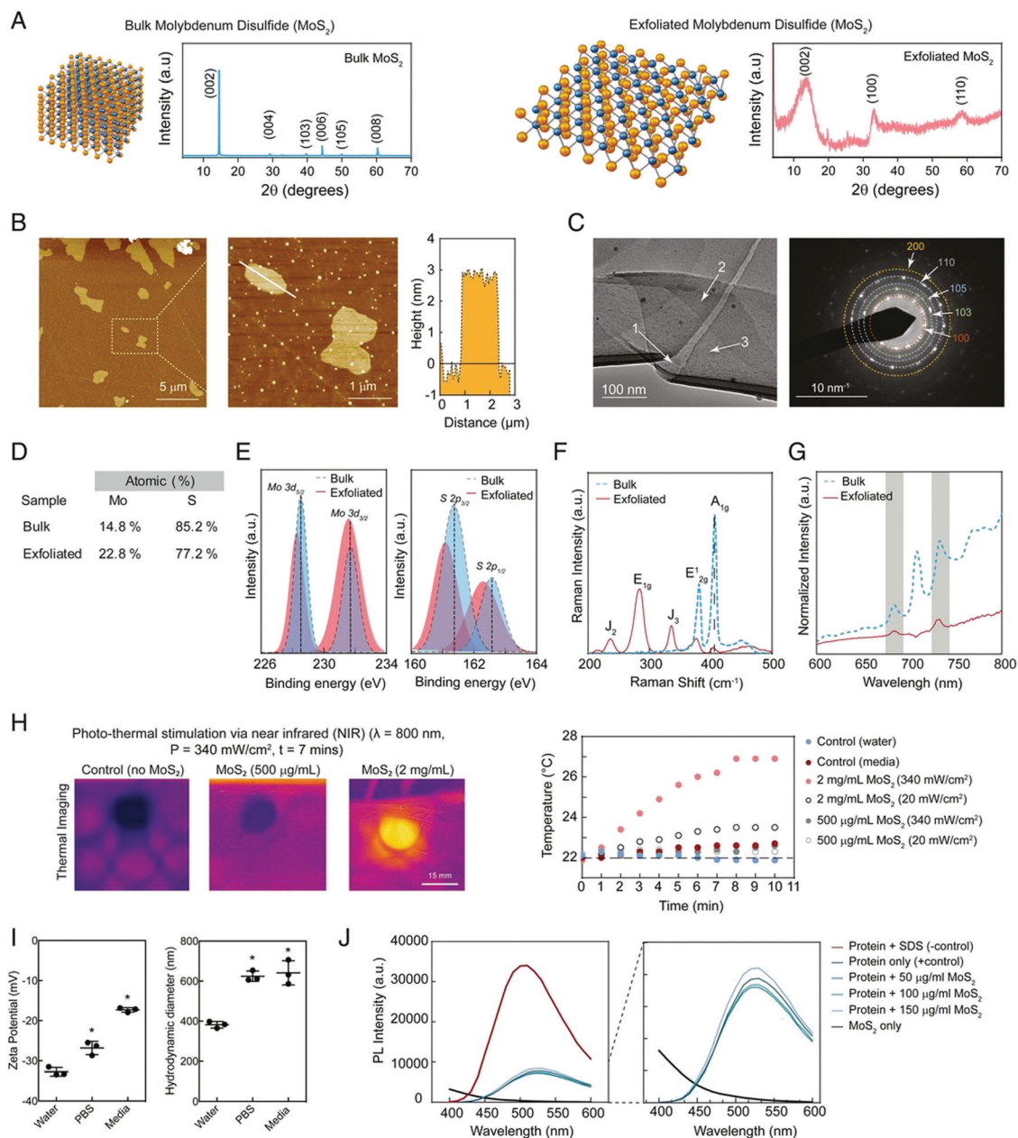
Fig. 3 Physicochemical characterization of exfoliated 2D MoS 2 nanosheets. (A) X-ray diffractogram of bulk and exfoliated MoS 2 , (B) atomic force microscopy (AFM) for confirming the 2D shape, (C) transmission electron microscopy (TEM) images of ultrathin MoS 2 sheets along with electron diffraction pattern, (D) atomic composition of bulk and exfoliated MoS 2 determined via elemental analysis, (E) X-ray photoelectron spectroscopy (XPS) analysis, (F) Raman spectroscopy, (G) photoluminescent measurements, (H) response to near infra-red (NIR) light was determined using an infra-red (IR) camera and change in temperature over time, (I) zeta potential and hydrodynamic size of exfoliated MoS 2 in water, phosphate buffer saline (PBS), and media, and (J) 8-anilino-1-naphthalenesulfonic acid (ANS) assay shows protein structures are intact in the presence of exfoliated MoS 2 . 128
