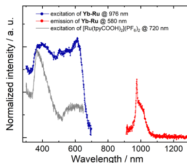
Fig. 5 Near-IR emission (red dot, \lambda_{\text{ex}} = 580 \text{ nm} ) and excitation (blue dot, \lambda_{\text{em}} = 976 \text{ nm} ) profiles of Yb-Ru solid powder, and the excitation profile (grey line, \lambda_{\text{em}} = 720 \text{ nm} ) of the [\text{Ru}(\text{tpyCOOH})_2](\text{PF}_6)_2 complex in the solid state.
