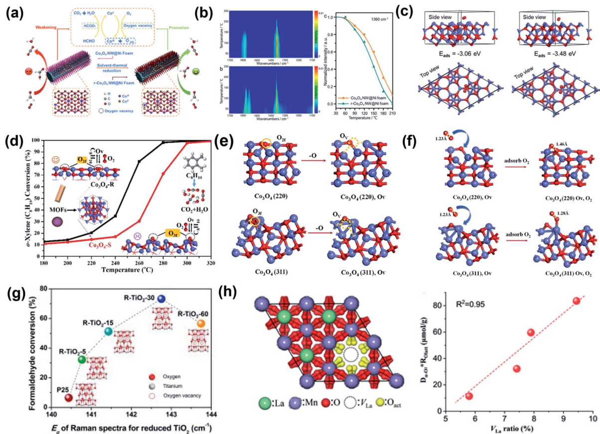
Fig. 21 (a) Schematic illustration of the catalytic oxidation of HCHO over r\text{-Co}_3\text{O}_4 NW@Ni with OV; (b) In situ DRIFTS after HCHO adsorption over \text{Co}_3\text{O}_4 NW@Ni and r\text{-Co}_3\text{O}_4 NW@Ni catalysts as a function of temperature. (c) \text{O}_2 molecule adsorbed on the (111) surface of \text{Co}_3\text{O}_4 NW@Ni foam and r\text{-Co}_3\text{O}_4 NW@Ni catalysts. Adapted with permission from ref. 293 Copyright (2020) American Chemical Society. (d) Catalytic oxidation activities of o -xylene over MOF-derived \text{Co}_3\text{O}_4 with different shapes. (e) OV formation over the (220) and (311) surfaces of \text{Co}_3\text{O}_4 , respectively; (f) side view of the adsorption configuration of \text{O}_2 over the (220) and (311) surfaces of \text{Co}_3\text{O}_4 with OV. The Co and O atoms are in blue and red, respectively. Adapted with permission from ref. 294 Copyright (2021) American Chemical Society. (g) Formaldehyde conversion over reduced \text{TiO}_2 of different OV concentrations. Adapted with permission from ref. 296 Copyright (2019) Elsevier. (h) Activation of surface lattice oxygen induced by La vacancies and the amount of released surface \text{O}_{\text{latt}} ( D_{\alpha\text{-O}_2} \text{RO}_{\text{latt}} ) as a function of V_{\text{La}} ratio. Adapted with permission from ref. 297 Copyright (2021) Wiley-VCH Verlag GmbH & Co. KGaA.
