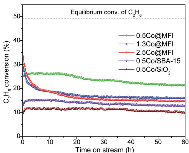
Fig. 5 Effect of Co loading and catalyst support on the EDH activities of different Co catalysts. Reaction conditions: 100 mg catalyst, pretreatment by 10% H_2/N_2 for 30 min, 20% C_2H_6/N_2 , 10 mL min^{-1} , 1 bar, 650 °C.
