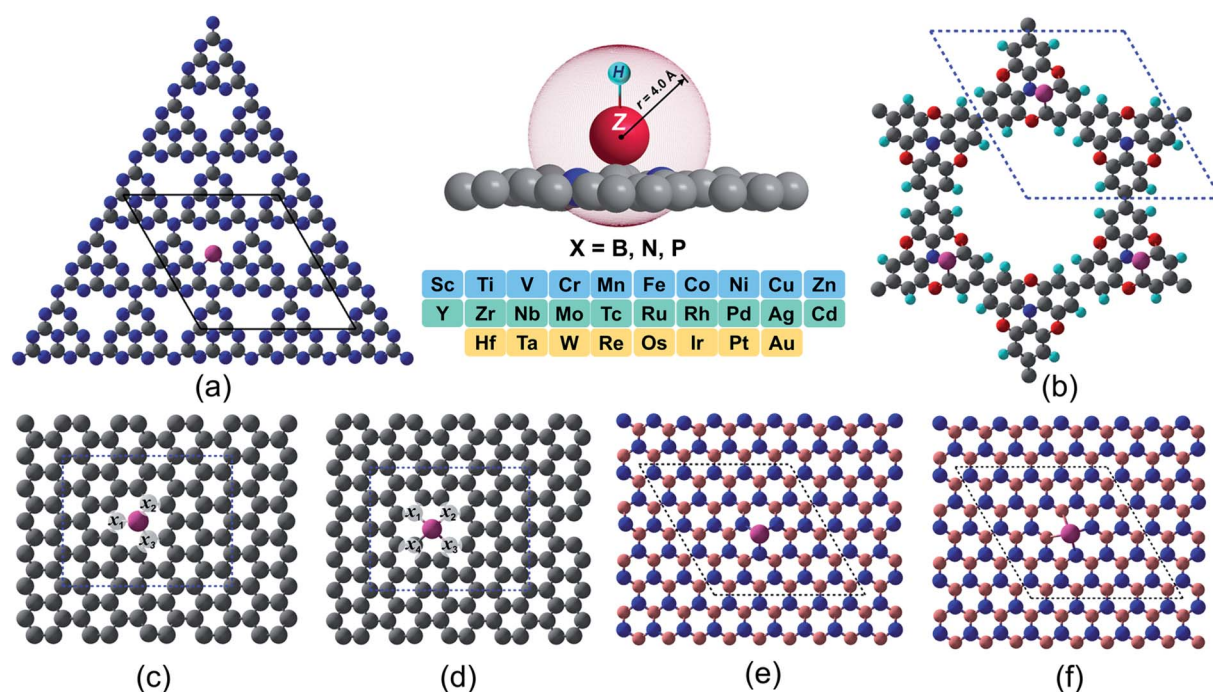
Fig. 1 Proposed 2D materials with TM embedded at various defect sites. (a) g\text{-}C_3N_4 (b) 2DCP (c) graphene with one C defect site (d) graphene with two C defects site (e) h\text{-}BN with one B defect site (f) h\text{-}B_2N_2 with one B and one N defects site. The labeled sites ( x_1 – x_4 ) in light gray color in (c) and (d) represent the non-metal (B, N, P) doping sites in single and dual type doping fashion. Color code: metal, magenta; B, light pink; N, blue; C, gray; O, red; H, cyan.
