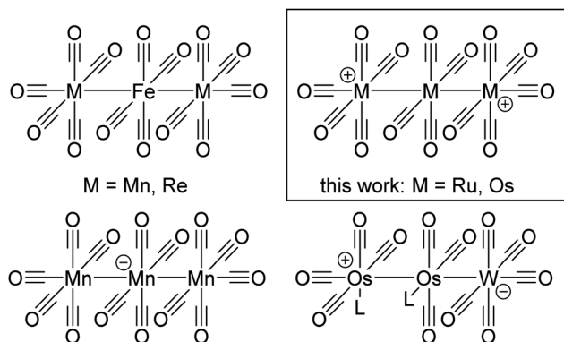
Fig. 5 Overview of known and new trimetal tetradeccarbonyls and their relatives.
