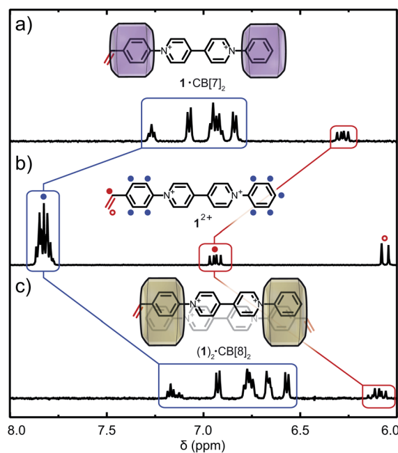
Fig. 2 Supramolecular complexation of 1^{2+} and CB[ n ]. 1 H NMR spectra of 1^{2+} at (a) \chi_{\text{CB}[7]} = 2 , (b) \chi_{\text{CB}[n]} = 0 and (c) \chi_{\text{CB}[8]} = 1 in \text{D}_2\text{O} . Cl - counter-ions are omitted for clarity.
