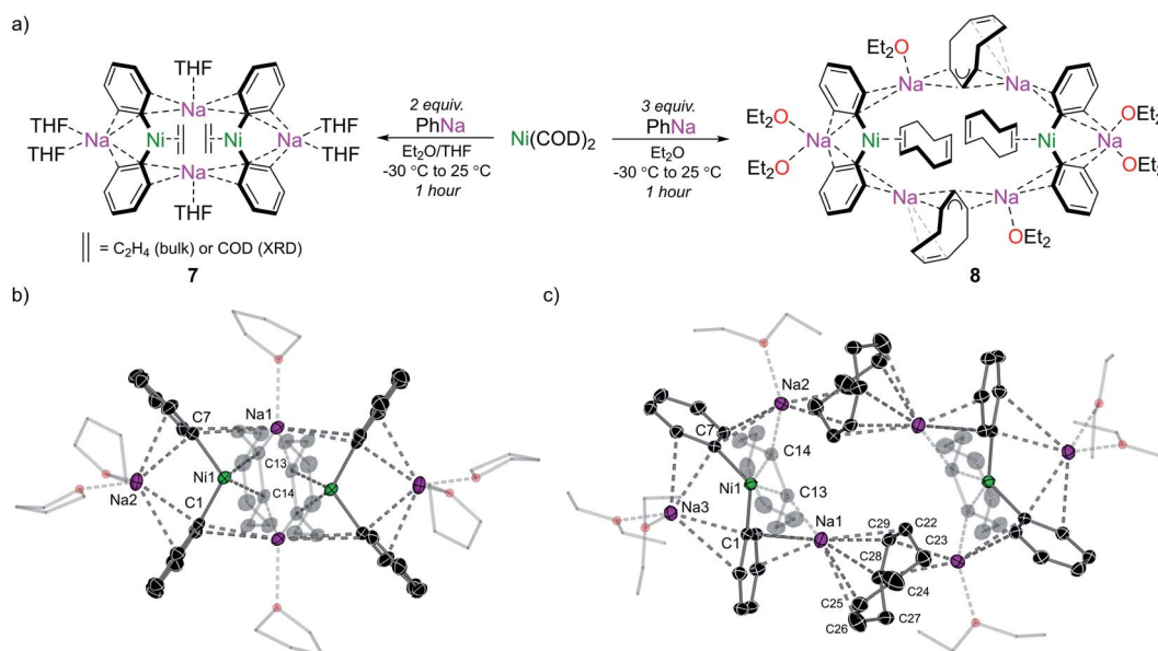
Fig. 7 (a) Reactions of Ni(COD)_2 with PhNa for the synthesis of [Na_2(THF)_3Ph_2Ni(olefin)]_2 ( 7 ) and identification of [Na_2(Et_2O)_3Ph_2(-NaC_8H_{11})Ni(COD)]_2 ( 8 ); (b) solid-state structure of 7 . Thermal ellipsoids shown at 30% probability. Hydrogen atoms omitted and THF rings drawn as wireframes for clarity; (c) solid-state structure of 8 . Thermal ellipsoids shown at 30% probability. Hydrogen atoms omitted and Et groups drawn as wireframes for clarity.
