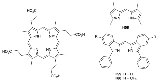
Scheme 22 Structures of the porphyrin H 2 CPI, and three Hbdipyrrin ligands.
