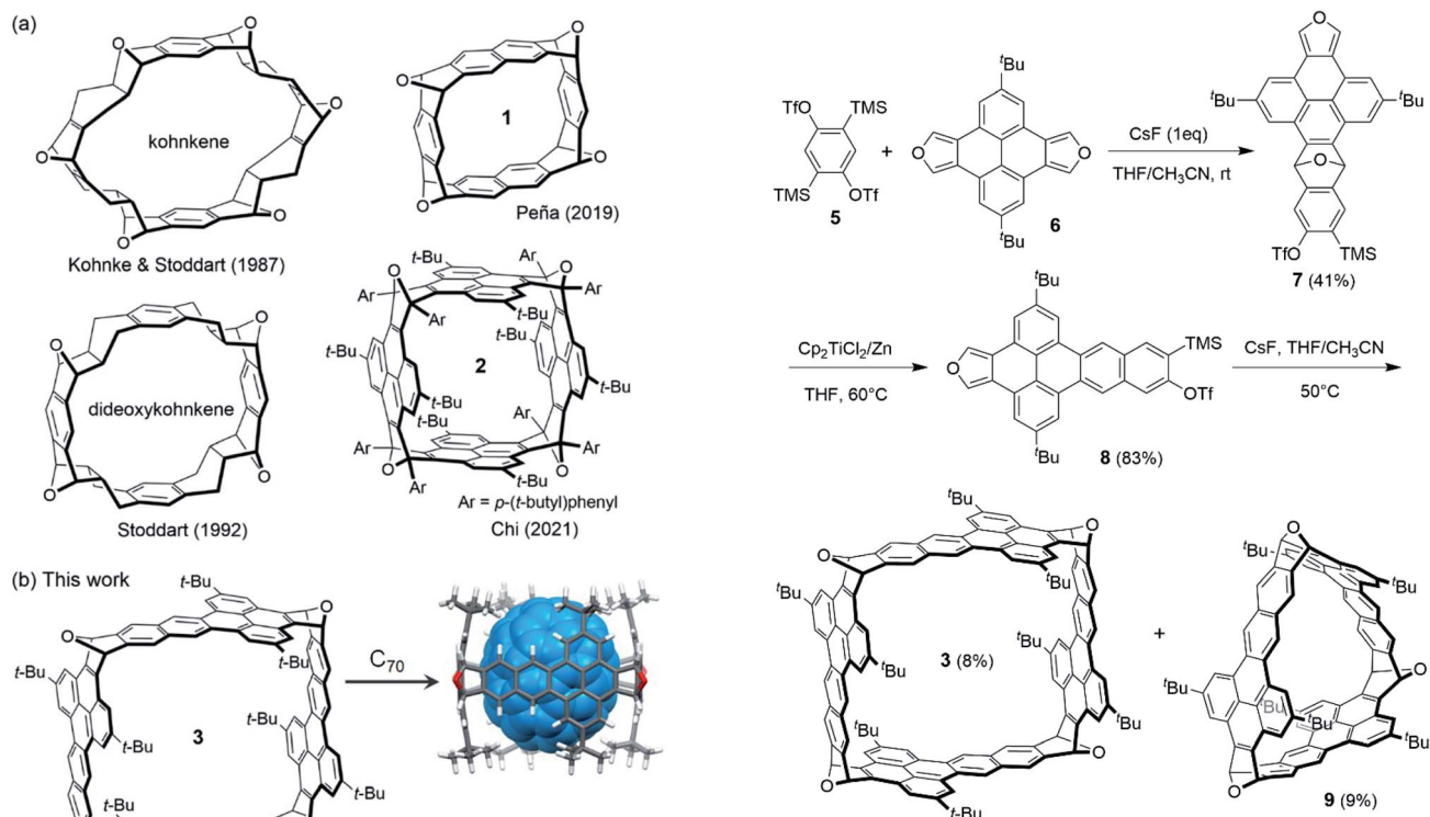
Scheme 1 Synthesis of 3.
