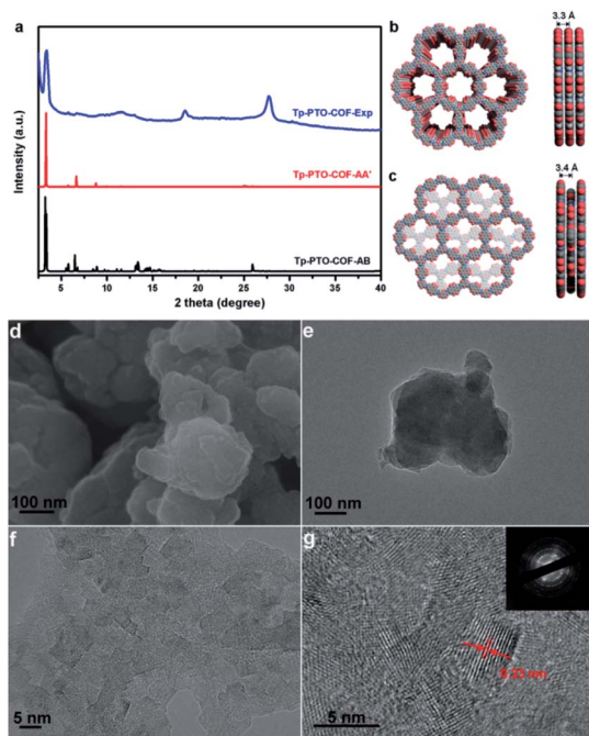
Fig. 2 (a) Comparison of the PXR patterns among the as-synthesized structure (blue), the simulated eclipsed AA structure (red), and the simulated staggered AB structure (black); (b) simulated eclipsed AA structure of Tp-PTO-COF; (c) simulated staggered AB structure of Tp-PTO-COF; (d) SEM image of Tp-PTO-COF; (e) TEM image of Tp-PTO-COF; (f and g) HRTEM images of Tp-PTO-COF. The inset is the corresponding SAED image.
