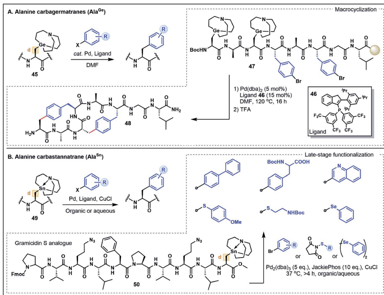
Fig. 7 Ala umpolung strategies. (A) Overview of Ala carbagermatrane derivatives and their use in peptide macrocyclization. (B) Overview of Alacarbastannatrane derivatives and their applications in late-stage functionalization.
