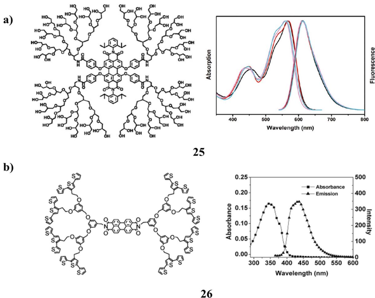
Fig. 17 (a) Structure of water-soluble perylene diimide core dendrimer (25). (b) Electropolymerizable terthiophene-based poly(aryl ether) dendrimer (26).
