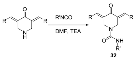
Scheme 12 Synthetic route towards 3,5-bis(ylidene)- N -substituted-4-piperidone-1-carboxamides 32 .
