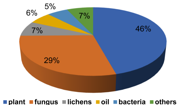
Fig. 3 Natural products against drug resistant bacteria from diverse terrestrial sources.
