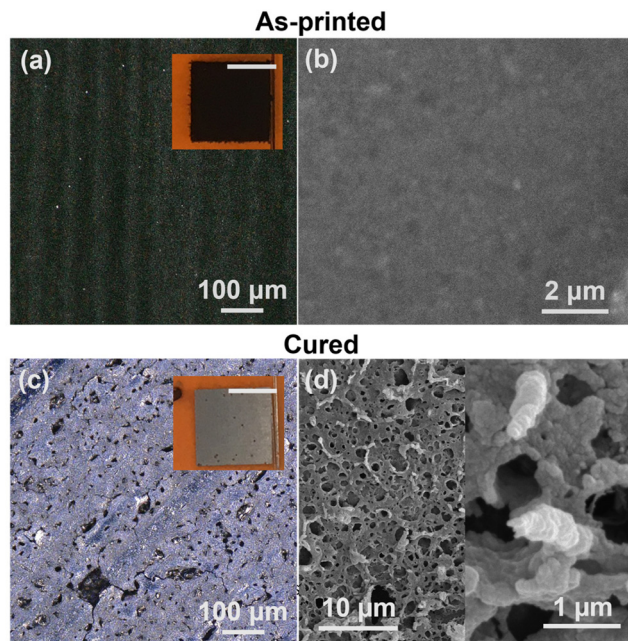
Fig. 5 Morphology of the print \text{TiH}_2 , including (a and c) optical and (b and d) SEM imaging for as-printed (a and b) and photonicallly cured (c and d) films.
