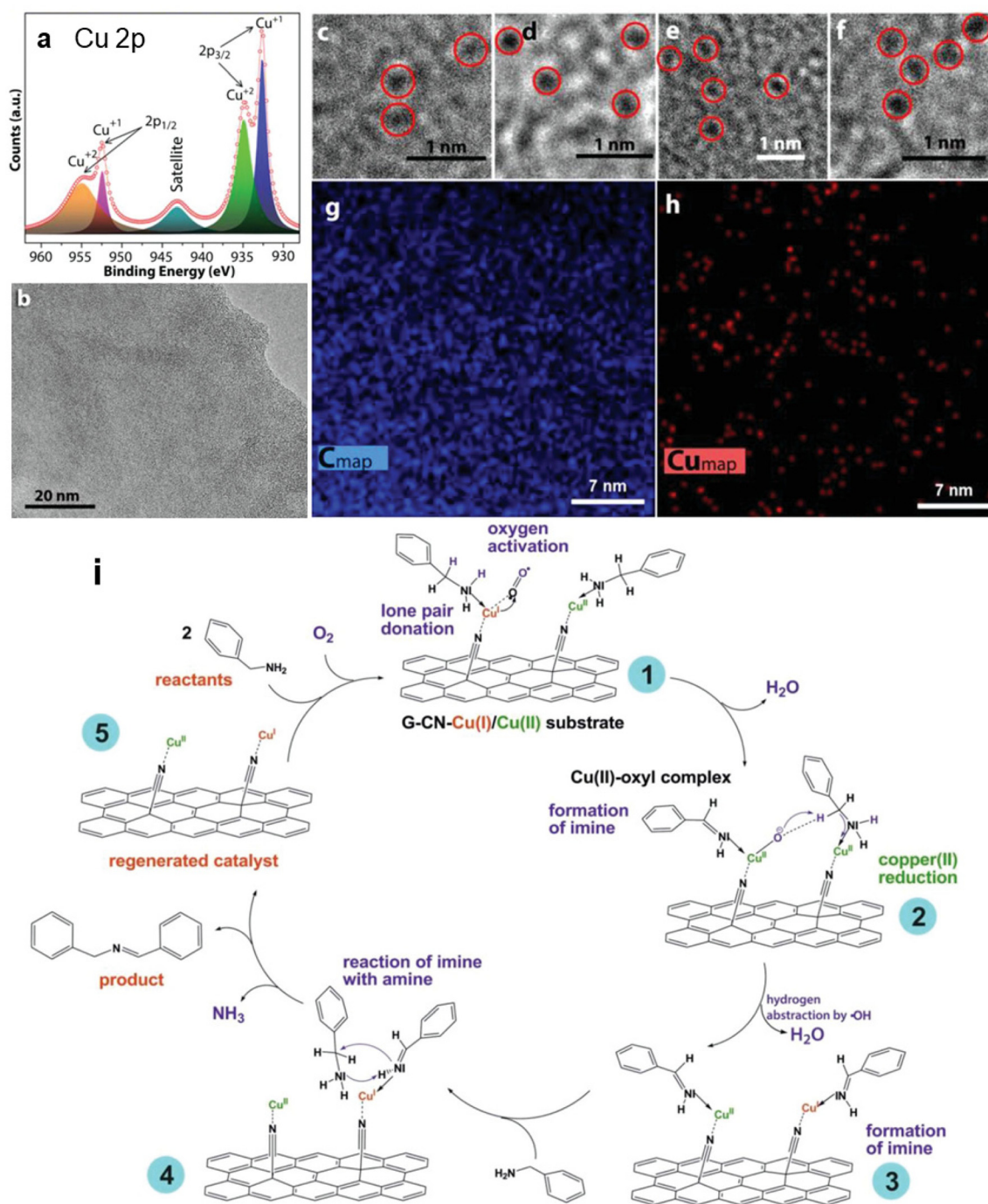
Fig. 3 (a) HR-XPS Cu 2p spectrum of the Cu(II)/Cu(I)···GCN catalyst. (b) HRTEM image of representative Cu(II)/Cu(I)···GCN flake. (c–f) Representative high magnification HR-TEM images from the catalyst showing high-contrast spots originating from embedded copper atoms (c and d) before and (e and f) after the catalytic reaction. EDS chemical mapping of the Cu(II)/Cu(I)···GCN catalyst for (g) C and (h) Cu. (i) Mechanism of the catalytic cycle of amine coupling reaction using Cu(II)/Cu(I)···GCN catalyst. This figure has been adapted from ref. 12 with permission from the John Wiley and Sons, copyright 2019.
