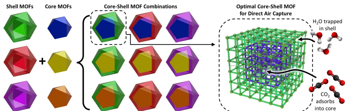
Fig. 1 Overview of the strategy for designing optimal core-shell MOFs for DAC. A library of MOFs is combinatorially assembled into all of the possible core-shell MOF pairs, and then each pair is computationally evaluated to find candidates for experimental synthesis. Optimal designs should prevent H 2 O from reaching the core while allowing for significant CO 2 adsorption in the core. Note that we include in our consideration core-shell MOF “pairs” where the core and the shell are the same MOF.
