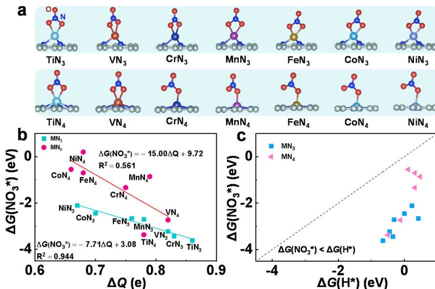
Fig. 2 (a) Atomic configurations of the \text{TMN}_3\text{@G} (upper panel) and \text{TMN}_4\text{@G} (lower panel) with the adsorbed \text{NO}_3^- . (b) The relationship between charge transfer ( \Delta Q ) of the \text{NO}_3^- and its binding free energy ( \Delta G(\text{NO}_3^*) ). (c) Comparison of the binding free energies of \text{NO}_3^- ( \Delta G(\text{NO}_3^*) ) and H atom ( \Delta G(\text{H}^*) ).
