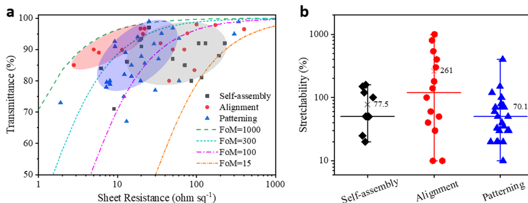
Fig. 18 (a) Transmittance versus sheet resistance of the MNW-based TEs fabricated by self-assembly, 34,36,45,47–49,108,131,134,327,353–357 alignment, 12,28,29,53,77,79,81,86,88,91,95,96,102,160,170,358,359 and patterning methods. 37,105,145,216,217,219,220,223,230,234,238,241,244,249,259,262,263,281,305,308,314,315,317,324,335,340,360–364 The dotted lines derived from eqn (6) denote the performances at different FoMs. (b) Stretchability of the MNW-based SEs fabricated by self-assembly, 34,36,124,131,365–371 alignment, 29,77,82,87,89,167,358,372–376 and patterning methods. 37,139,232,244,251,259,283,293,308,315,317,340,361
