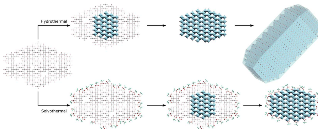
Scheme 1 Hydrothermal treatment of amorphous titania leads to intraparticle crystallisation of the anatase phase and subsequent growth by interparticle fusion, while solvothormal treatment in trifluoroacetic acid initially leads to complete surface modification with intraparticle crystallisation yielding surface capped anatase phase hybrid nanocrystals.
