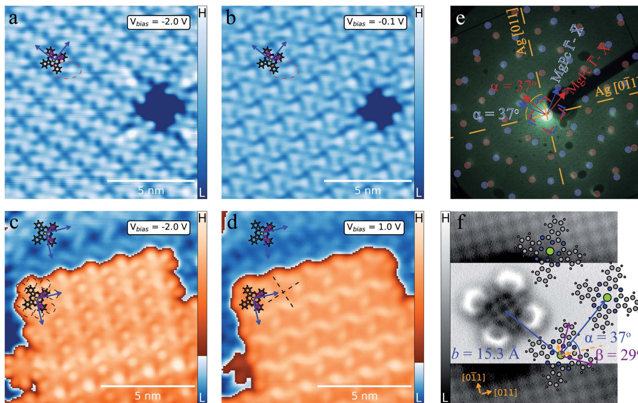
Fig. 1 MgPc monolayer (ML) and bilayer (2L) self-assemblies on Ag(100). (a)–(d) STM topographies of ML [ I_t = 100 pA, V_{\text{bias}} = -2.0 V (a) and V_{\text{bias}} = -0.1 V (b)] and 2L [ I_t = 100 pA, V_{\text{bias}} = -2 V (c) and V_{\text{bias}} = 1 V (d)] with MgPc chemical structure superimposed (grey: carbon; blue: nitrogen; white: hydrogen; green: magnesium). Blue arrows: unit cell vectors \mathbf{b}_1 and \mathbf{b}_2 of 2D square molecular lattice (lattice constant: b = \|\mathbf{b}_1\| = \|\mathbf{b}_2\| = 1.53 \pm 0.02 nm). Violet arrows: MgPc isoindole axes. (e) LEED pattern (electron energy: 25.5 eV) of MgPc ML. Orange dashed lines: Ag(100) high-symmetry directions. Superimposed blue and red dots correspond to LEEDPat 43 simulation for MgPc arrangement within ML, consistent with STM data (with \pm 37^\circ angle between MgPc self-assembly and Ag(100) high-symmetry directions). Dashed blue and red squares: Brillouin zone boundaries of equivalent, mirror-symmetric MgPc ML configurations. LEED image with no annotation available in Fig. S5 of ESI.† (f) Constant-height nAFM image of single MgPc, including Ag(100) atomic resolution for MgPc registration [STM setpoint: V_{\text{bias}} = 1.5 mV, I_t = 10 pA on MgPc; V_{\text{bias}} = 1.5 mV, I_t = 220 pA on Ag(100)], with superimposed MgPc chemical structure consistent with ML MgPc arrangement given by STM (a) and (b) and LEED (e). MgPc isoindole axes (violet) and MgPc superlattice unit cell vectors (blue) are rotated by 29^\circ and 37^\circ , respectively, relative to Ag(100) unit cell vectors (orange arrows).
