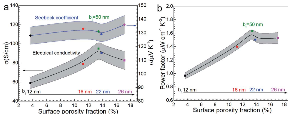
Fig. 8 (a) The electrical conductivity \sigma and the Seebeck coefficient \alpha and (b) power factor \alpha^2\sigma of nanoporous \text{Ca}_3\text{Co}_4\text{O}_9 films as function of surface porosity fraction at room temperature.
