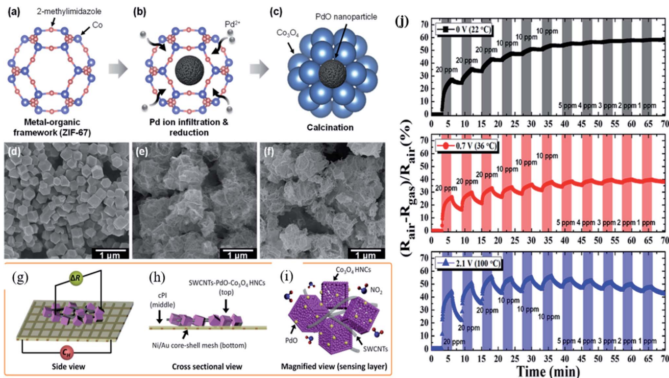
Fig. 13 (a–c) Schematic diagram of PdO loaded \text{Co}_3\text{O}_4 Pd/ZIF-67 after annealing at 400\text{ }^\circ\text{C} , (d–f) SEM image of ZIF-67, PdO-loaded \text{Co}_3\text{O}_4 HNCs after calcination, and SWCNT-loaded PdO- \text{Co}_3\text{O}_4 HNCs, (g–i) schematic illustration of the fabrication of the SWCNT-loaded PdO- \text{Co}_3\text{O}_4 HNC sensor device on a flexible conducting PI film (cPI) with a Ni/Au mesh heater based substrate, and (j) response transients of the SWCNT-loaded PdO- \text{Co}_3\text{O}_4 HNC sensor towards \text{NO}_2 at different applied voltages (0–2.1 V). Reprinted from ref. 122, copyright@2021, American Chemical Society.
