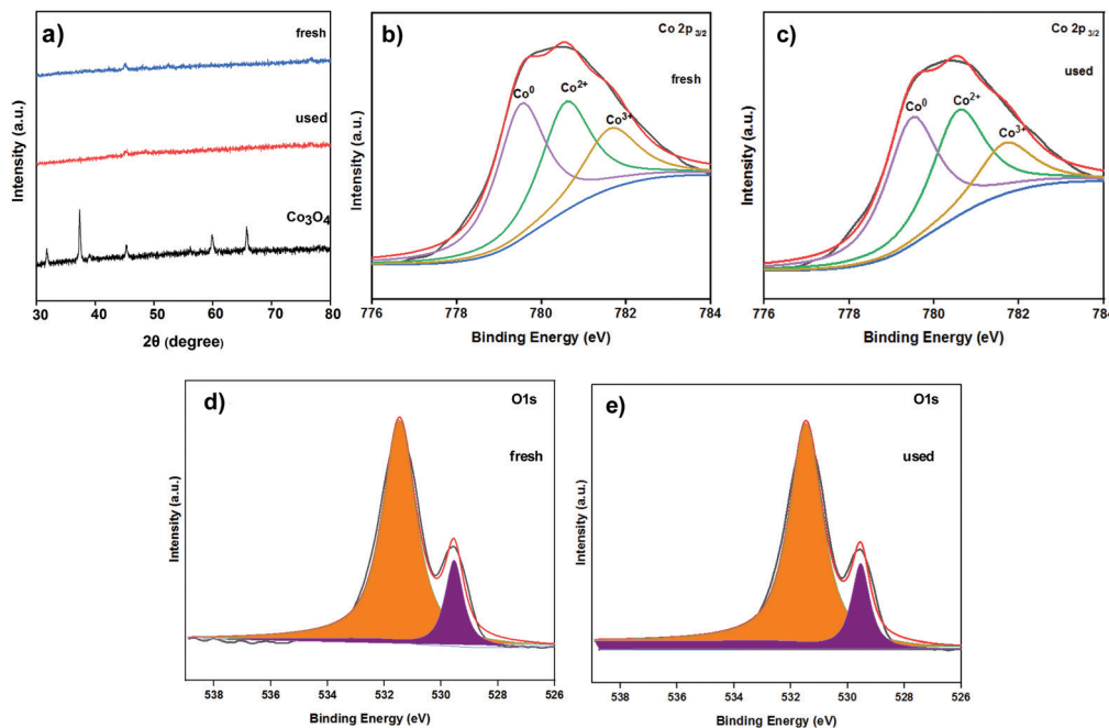
Fig. 12 The XRD pattern and XPS spectra of the Co catalysts. (a) The XRD pattern of fresh Co-400 catalyst, Co-400 catalyst after reuse 4 times, and commercial \text{Co}_3\text{O}_4 ; (b) Co 2\text{P}_{3/2} XPS spectra of fresh Co-400 catalyst; (c) Co 2\text{P}_{3/2} XPS spectra of Co-400 catalyst after reuse 4 times; (d) O 1\text{s} XPS spectra of fresh Co-400 catalyst; (e) O 1\text{s} XPS spectra of Co-400 catalyst after reuse 4 times.
