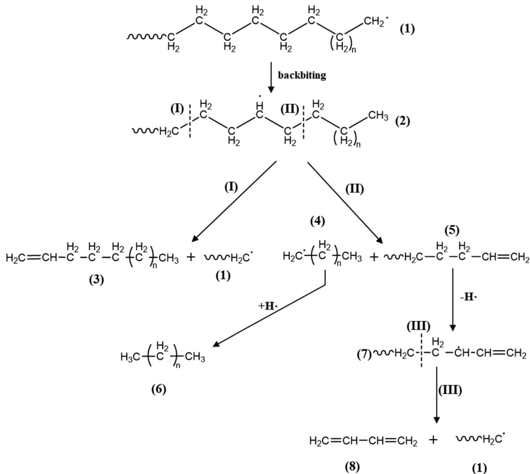
Scheme 1 Fundamental reactions for the thermal decomposition of PE leading to alkanes (6), alkenes (5) and alkdienes (8). Arabic numerals indicate chemical species that form during the pyrolysis of PE, while Roman numerals indicate the occurrence and position of the scission of chemical bond.
