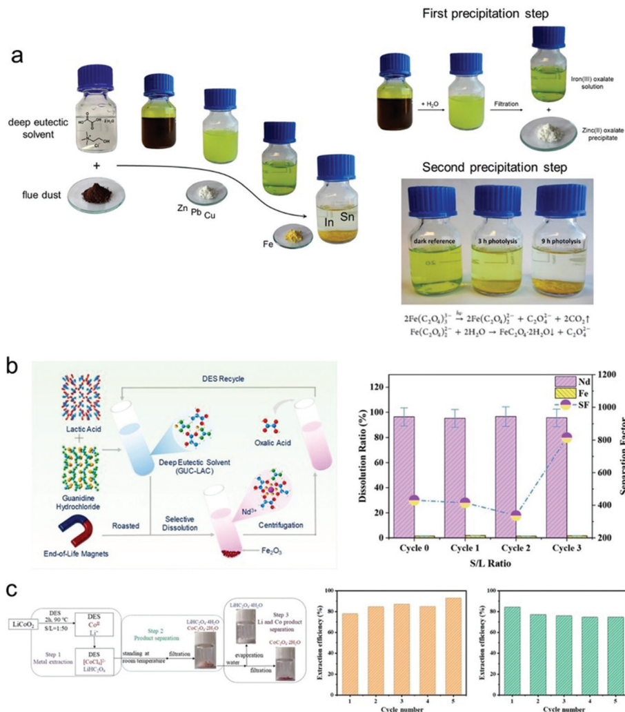
Fig. 9 (a) Schematic diagram of leaching and selective extraction of zinc, iron, indium, and tin using ChCl : oxalic acid DES-based two-step precipitation procedure (left); dilution of oxaline leachate and precipitation of white zinc oxalate next to the green-colored filtrate in the first precipitation step (upper right); photograph and reaction formulations of photolysis of iron(III) oxalate solution using a UV lamp in the second precipitation step (lower right). Reprint with permission from ref. 161. Copyright © 2019, American Chemical Society. (b) Schematic diagram of selectively leaching neodymium from end-of-life NdFeB permanent magnets by guanidine hydrochloride : lactic acid DES (left) and the recycling performance of the DES (right). Reprint with permission from ref. 130. Copyright © 2020, American Chemical Society. (c) Schematic diagram of the one-pot extraction process using ChCl : oxalic acid DES for the recovery of lithium and cobalt from LiCo 2 and the recycling performance of DES for Li extraction (middle) and Co extraction (right). Reprint with permission from ref. 163. Copyright © 2021, American Chemical Society.
