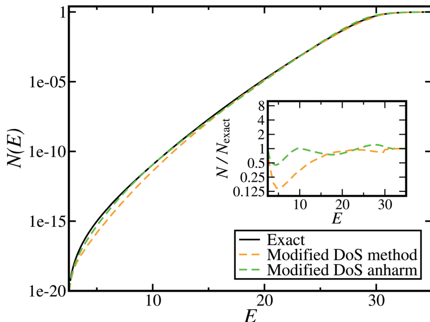
Fig. 6 A comparison of the exact cumulative reaction probability from the modified DoS method (eqn (88)) and the anharmonic-corrected modified DoS method (eqn (94)) for model 2, with V_{TS} = 20 , a_{eck} = 1 , a_{\omega} = \sqrt{2} , \omega_{TS} = 20 and \omega_r = 5 . The inset shows the relative error.
