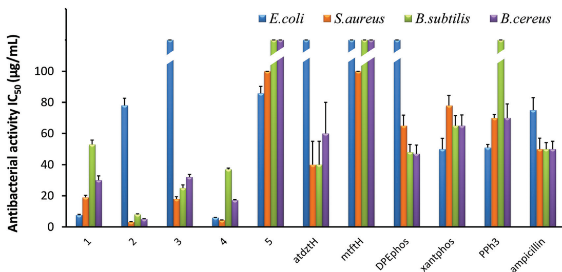
Fig. 3 In vitro antibacterial activity of 1–5, and their ligands atdztH, mfttH, DPEphos, xantphos, and PPh 3 in free form, expressed as half-minimum inhibitory concentration (IC 50 ) values ( \mu\text{g mL}^{-1} ) provided by a nonlinear curve fit-growth/sigmoidal-dose response on the experimental optical density data. Values are expressed as mean \pm standard deviation (SD) of three replicate measurements (with the exception of values higher than 100 \mu\text{g mL}^{-1} ).
